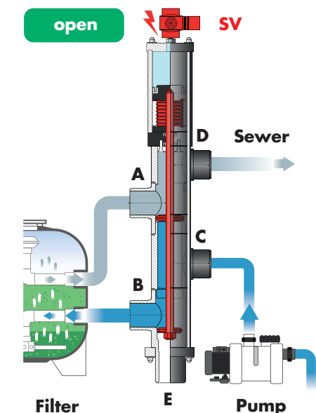
Backwash mode Solenoid valve open
