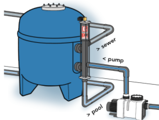
Fitted directly on the filter
