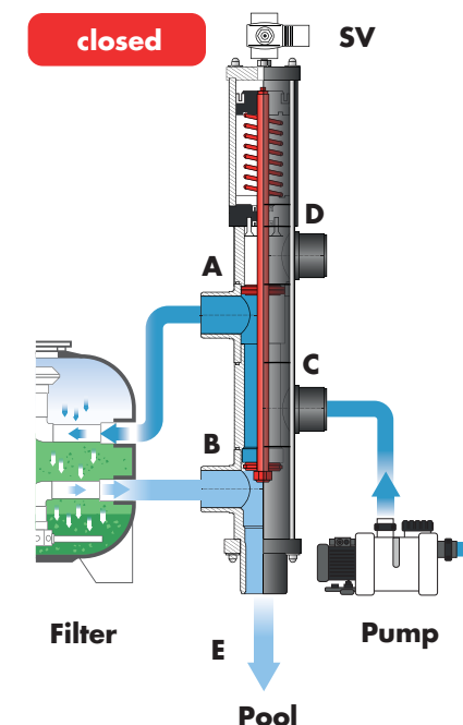
Filtration mode Solenoid valve closed
